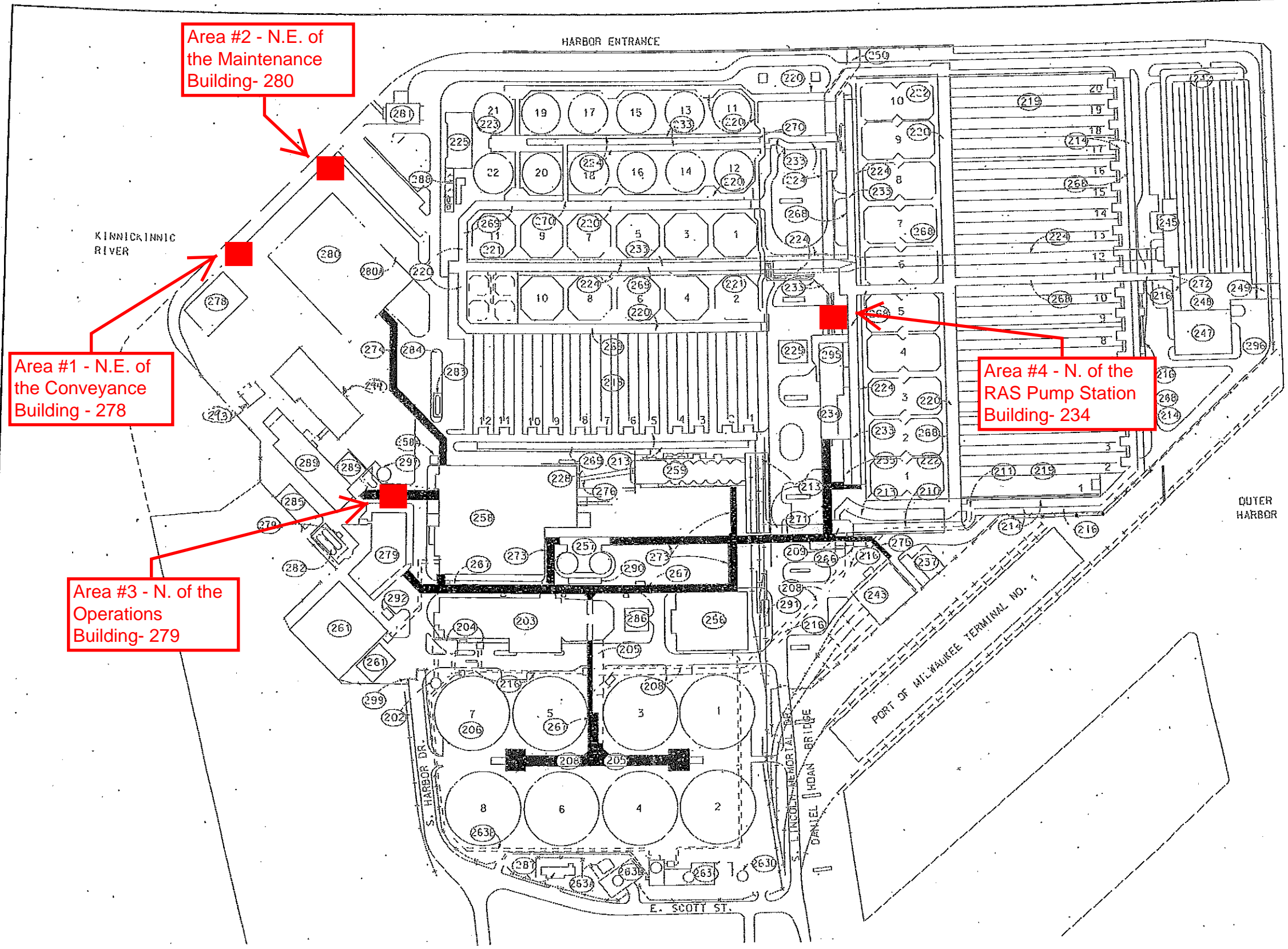
JONES ISLAND SITE PLAN 1"=120'
