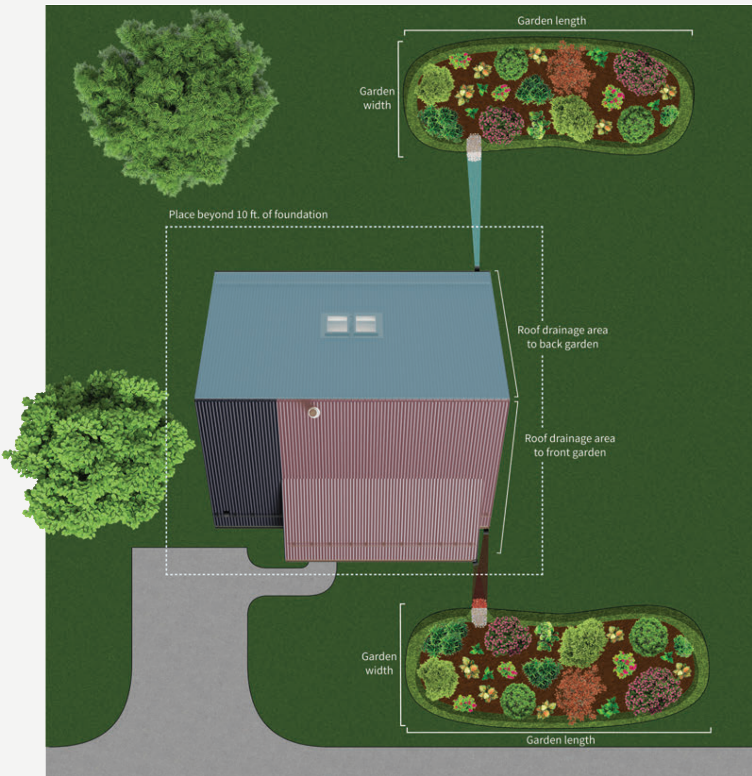
Figure 1. Displayed below is an example of two rain gardens placed in front and back of a property, highlighting the rain runoff areas on the roof. Pick a pleasing shape for the rain garden, like crescent, kidney, or teardrop shapes.
