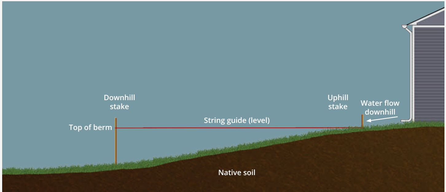
Figure 3. The string should be tied to the base of the uphill stake, then tied to the downhill stake at the same level.
