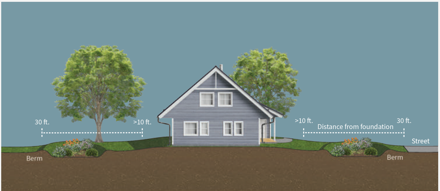
Figure 2. Rain gardens should be placed at least ten feet from the house and within thirty feet from the mouth of the downspout. Ideally, they should also be situated on a gentle slope that catches downspout water.
