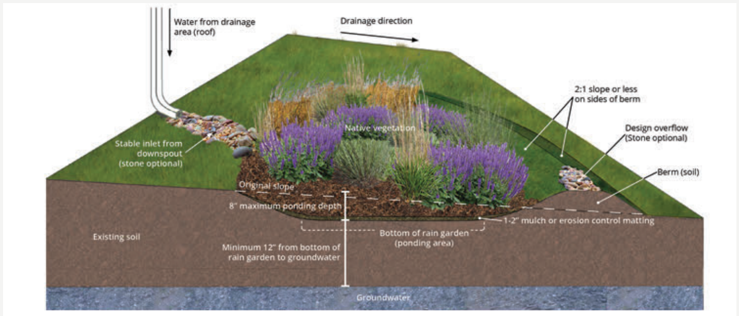
Figure 5. The top of the downhill part of the berm should come up to the same elevation as the entry to the rain garden at the uphill end.
